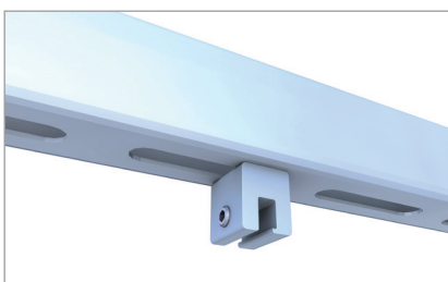
Centric load distribution in to the seam clamp
