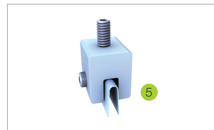
Clamp with VA saddle for copper standing seam roofs
